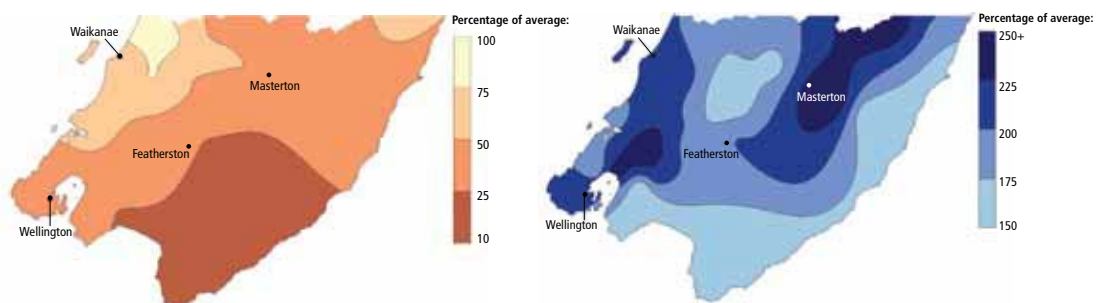
Rainfall as a percentage of average for the month during January (left) and February 2009 (right). Summer 2008/09 was a season of contrasts, with a very dry January, a wet February, and a return to low rainfall and river flows in March.
