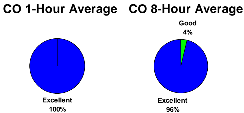
Figure 4.43: CO monitoring results at Masterton compared to air quality categories for the period October 2003 to October 2004
