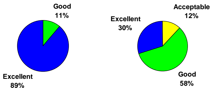
Figure 4.7: NO 2 monitoring results compared to air quality categories for the period October 2003 to October 2004
