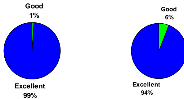
Figure 4.25: CO monitoring results compared to air quality categories for the period October 2003 to October 2004
